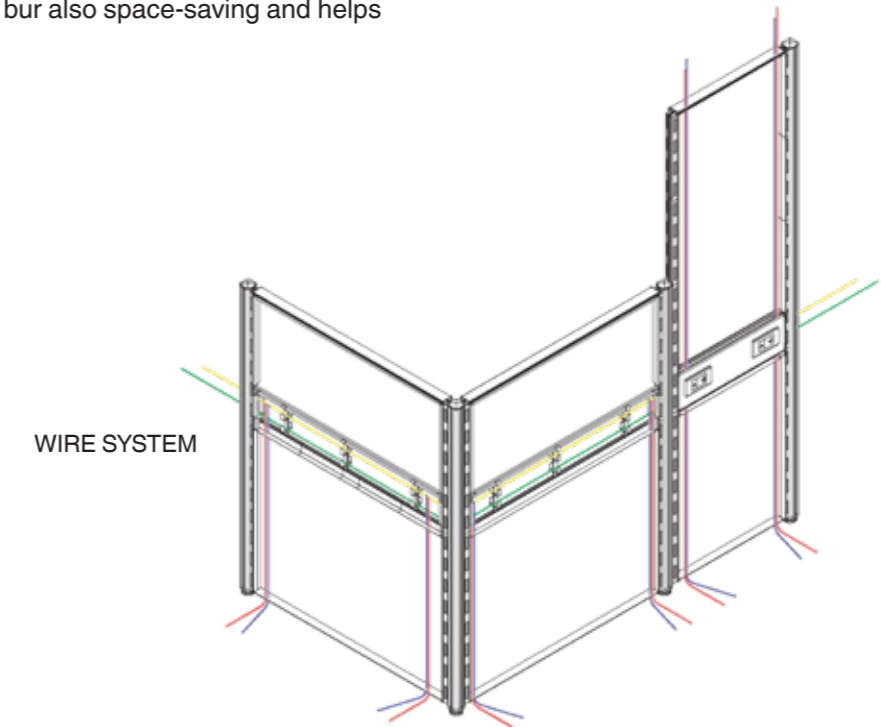
Electrical outlets are installed on the panel with utility channels.
